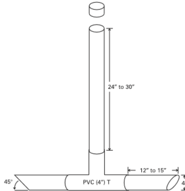
Figure 2. Inverted "T" homemade PVC bait station.
